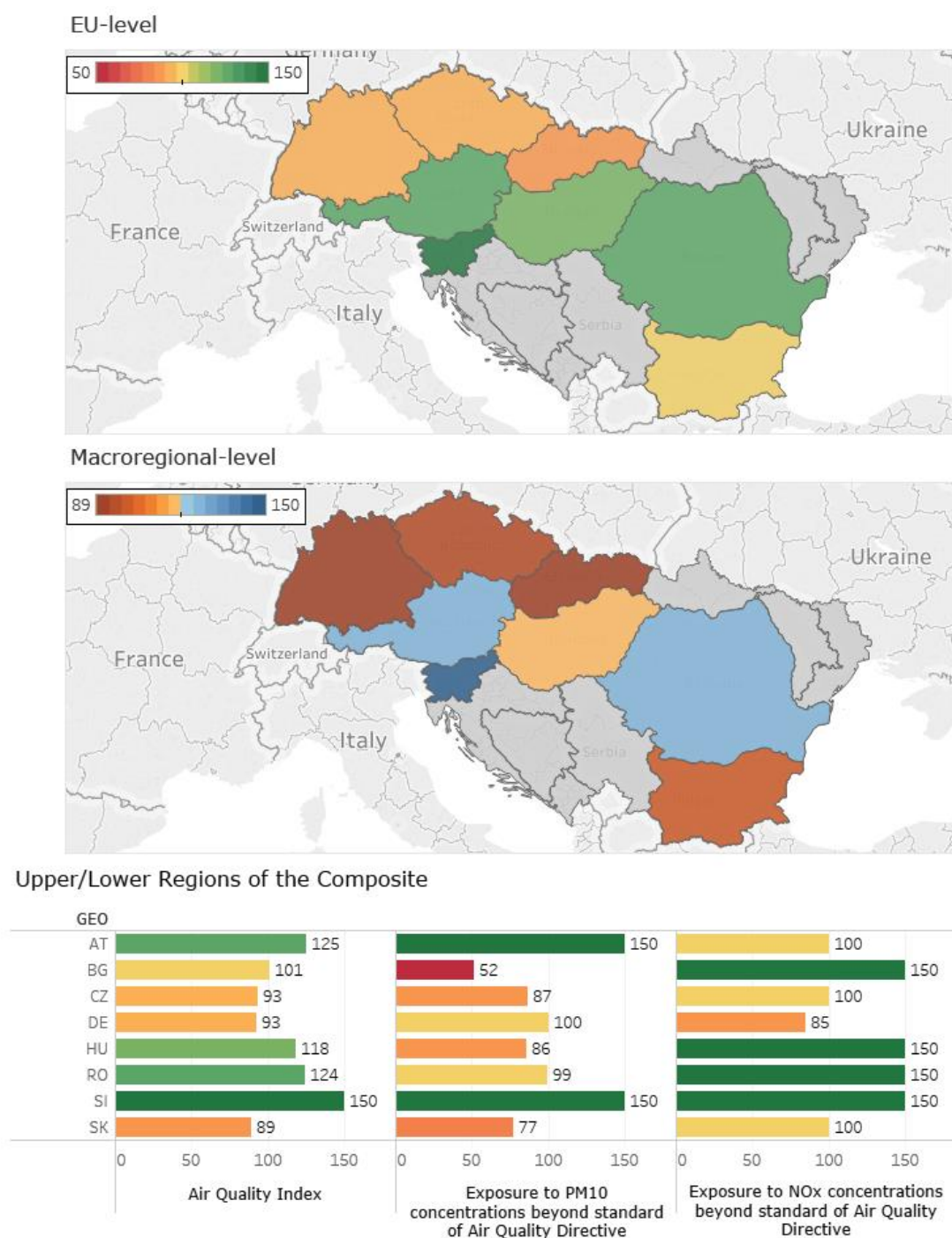
Figure 2-28: Air Quality Index by country in 2014, on an EU-wide (top) and Macro-regional (middle) comparison. The bottom figure shows the values for each country
