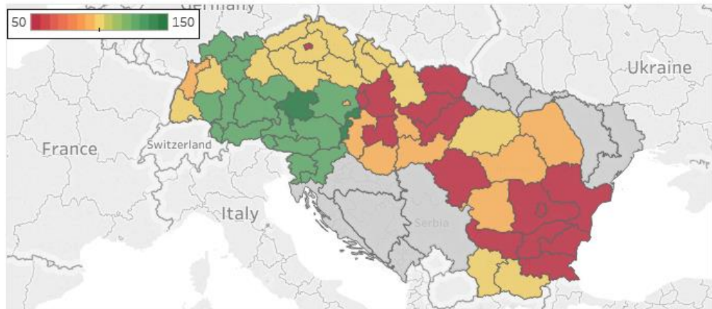
Figure 2-32: Shannon Evenness Index by NUTS-2 level regions in 2012, on an EU-wide (top) and Macro-regional (middle) comparison.
